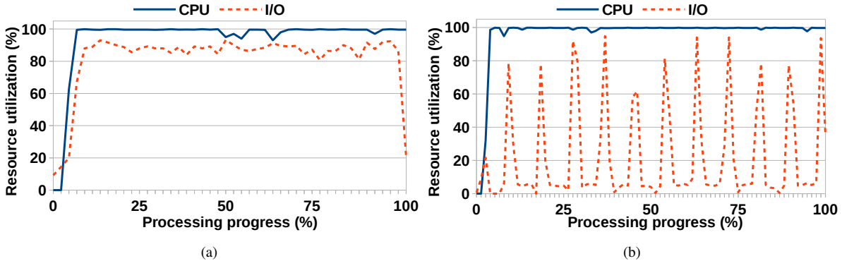
Figure 14: CPU and I/O utilization for resource-aware bi-level (a) and chunk-level (b) sampling.
