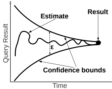
Figure 2: Online aggregation.
