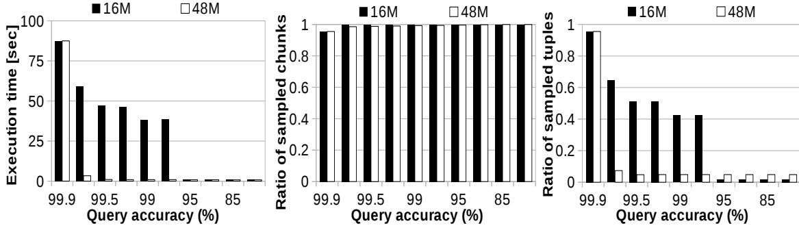
Figure 13: Sample synopsis effect on a sequence of queries with decreasing accuracy. For each accuracy, the query is executed two times.
