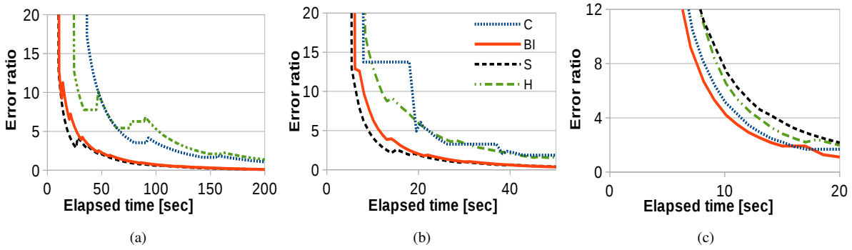
Figure 11: Sampling comparison as a function of the number of threads: 1 thread (a), 4 threads (b), and 16 threads (c).
