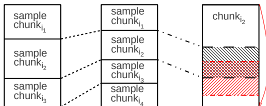
Figure 6: Maintenance of bi-level sample synopsis under new chunk insertion and existing chunk resampling.
