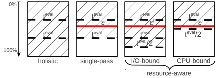
Figure 5: Bi-level sampling strategies in OLA-RAW.
