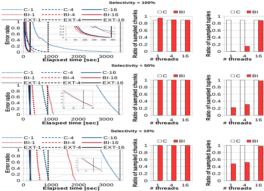
Figure 8: Results on the ptf-csv dataset.
