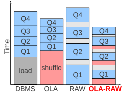
Figure 3: OLA-RAW approach.
