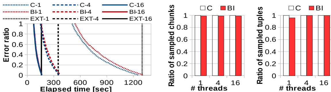
Figure 10: Results on the wiki dataset.
