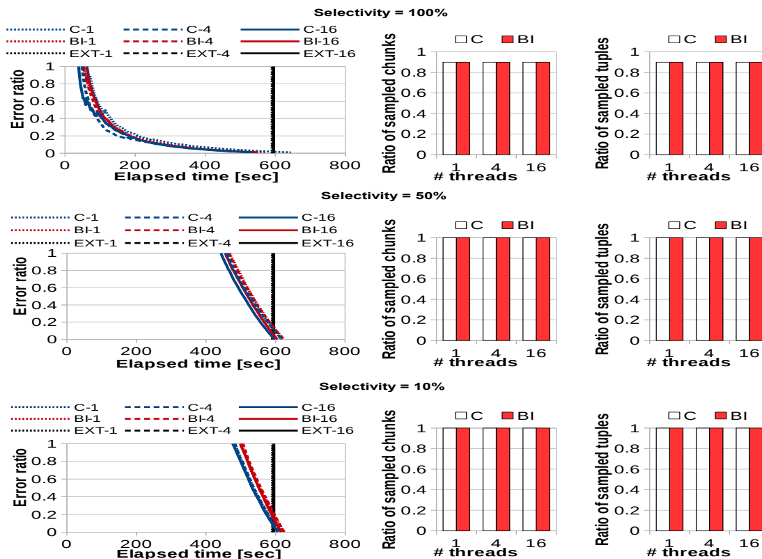
Figure 7: Results on the ptf-fits dataset.
