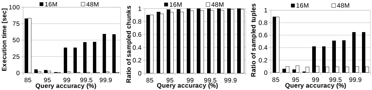
Figure 12: Sample synopsis effect on a sequence of queries with increasing accuracy. For each accuracy level, the query is executed two times.
