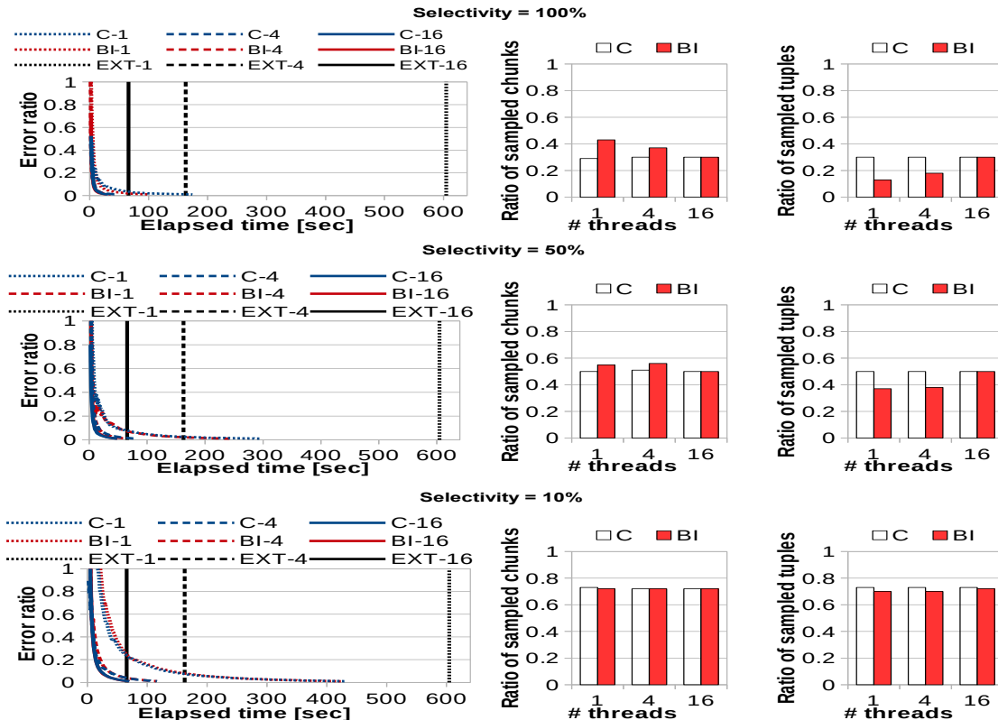
Figure 9: Results on the synthetic dataset.
