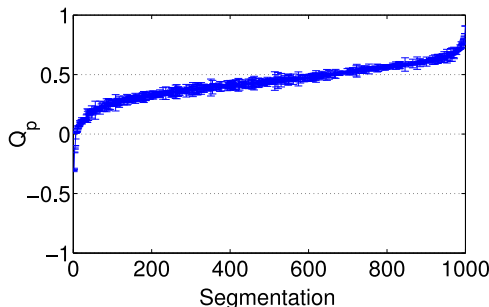
Fig. 13. Means and standard deviations of Q_p for 1,000 segmentations in our evaluation database. Error bars show the standard deviation of Q_p with respect to 50 random initial labelings. The results are sorted in ascending order of means.
