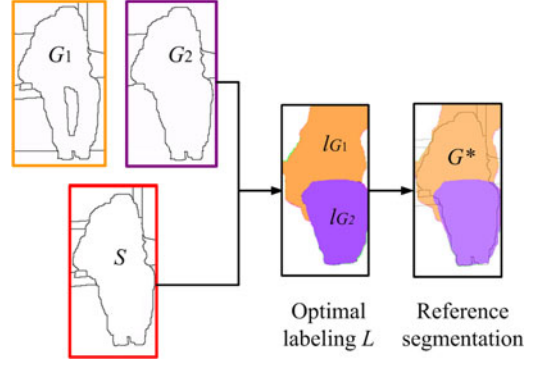
Fig. 3. An example to compose a reference segmentation for segmentation S with labeled segmentations G_1 and G_2 . The optimal labelings l_{G_1} , l_{G_2} of G_1 and G_2 generate a reference segmentation G^* , which matches S closely.
