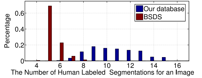
Fig. 9. Distribution of labeled segmentations in the proposed and BSDS500 datasets.
