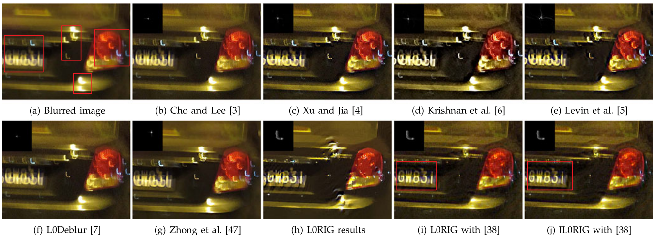
Fig. 13. Real blurry image with numerous saturated regions. The red boxes in (a) enclose some saturated pixels (e.g., highlighted blobs, streaks, and characters).
