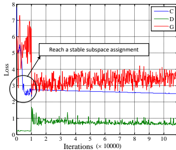
Fig. 4. Optimization losses of three modules, i.e. , C (blue), D (green) and G (red), over training iterations on the MNIST dataset. The \mathcal{L}_C demonstrates a downward trend before around 10,000-th iteration. Sequentially, the training of G and D is unstable, e.g. , D can easily discriminate the fake images from the real one so that the \mathcal{L}_D is low. After C reaches a stable subspace assignment, the framework begins a normal adversarial training of G , D and C .
