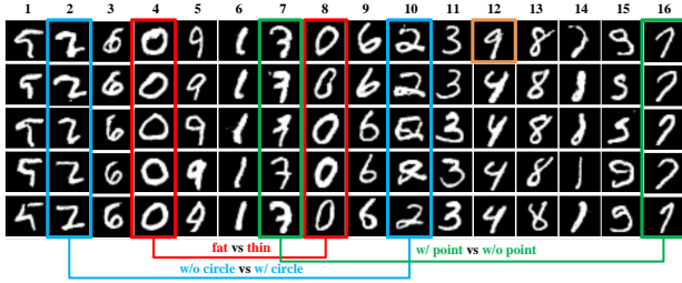
Fig. 3. Samples generated from joint unsupervised training on the MNIST dataset using the proposed Sub-GAN. Here, we set K = 16 ( top row ) to disentangle diverse subspaces \{\mathcal{S}_i\}_{i=1}^{16} . Note we construct this figure according to the sequence derived from the clusterer C . The bottom illustrates three pairs of different writing styles of digits 2, 0 and 7. The Sub-GAN can discover not only the 10 subspaces with the digits 0 – 9, but the different writing style, e.g. , the fat and thin ‘0’ in the 4-th and 8-th, respectively. The brown box reflects the failure case which confuses between 4 and 9.
