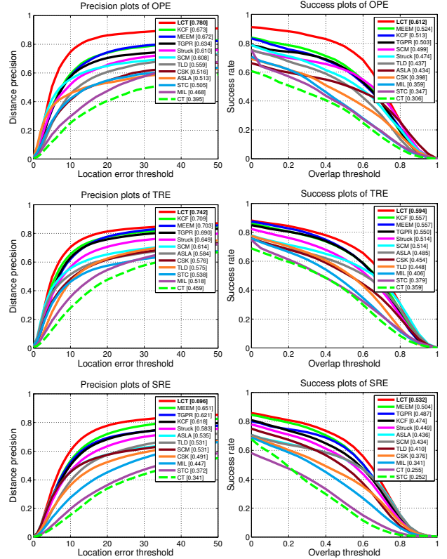
Figure 5. Distance precision and overlap success plots over 50 benchmark sequences using one-pass evaluation (OPE), temporal robustness evaluation (TRE) and spatial robustness evaluation (SRE). The legend contains the area-under-the-curve score for each tracker. The proposed LCT method performs favorably against the state-of-the-art trackers.
