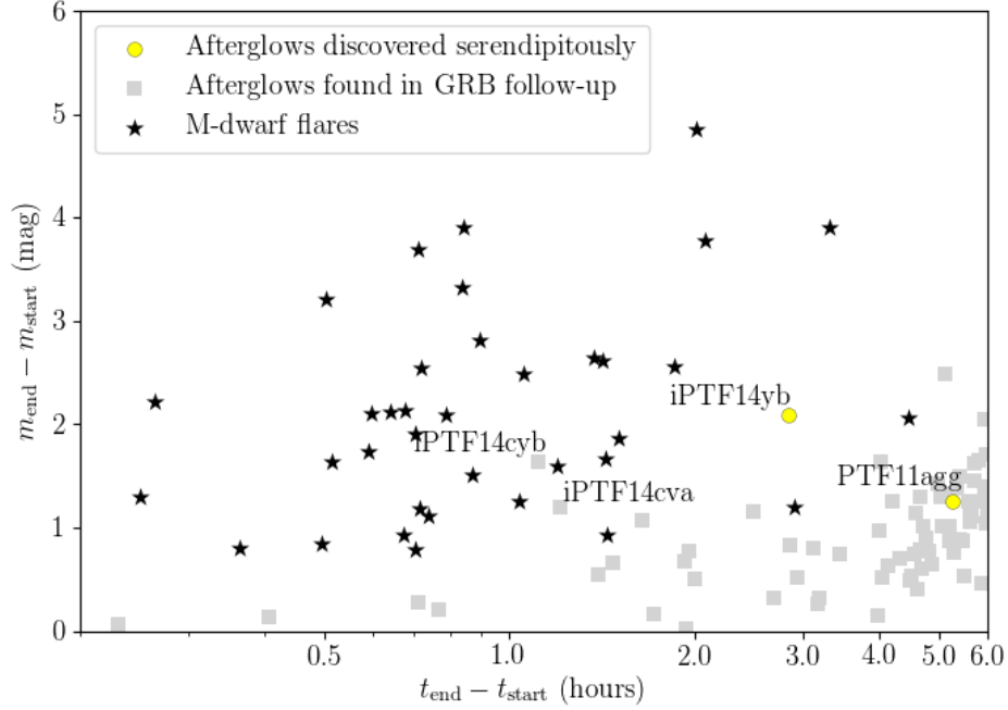
Figure 1. The (\Delta t, \Delta m) for the 40 candidates that show significant ( 5\text{-}\sigma ) intra-night fading (asteroids and artifacts of bad subtractions have been removed). The grey unlabeled points are a sample of GRB afterglows from Kann et al. (2010), sampled at 3 hours and 9 hours post-peak. For candidates with > 2 points in their light curves, we show the change in magnitude from the first observation to the last observation: \Delta t = t_{\text{end}} - t_{\text{start}} and \Delta m = m_{\text{end}} - m_{\text{start}} . M-dwarf flares typically fade faster and are detected in Pan-STARRS (see Table 2) with a characteristic red color. Thus, in our sample, filtering out sources with red hosts exclusively identifies iPTF14yb, the GRB discovered serendipitously by iPTF, as well as two afterglows found in follow-up to Fermi GRB triggers. PTF11agg is shown for reference. There is one M-dwarf with a \Delta t below the lower limit on the plot.
