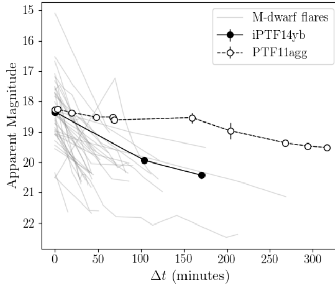
Figure 2. r -band light curves for the 37 M-dwarf flares in our sample (grey, background) overlaid with light curves of iPTF14yb and PTF11agg
