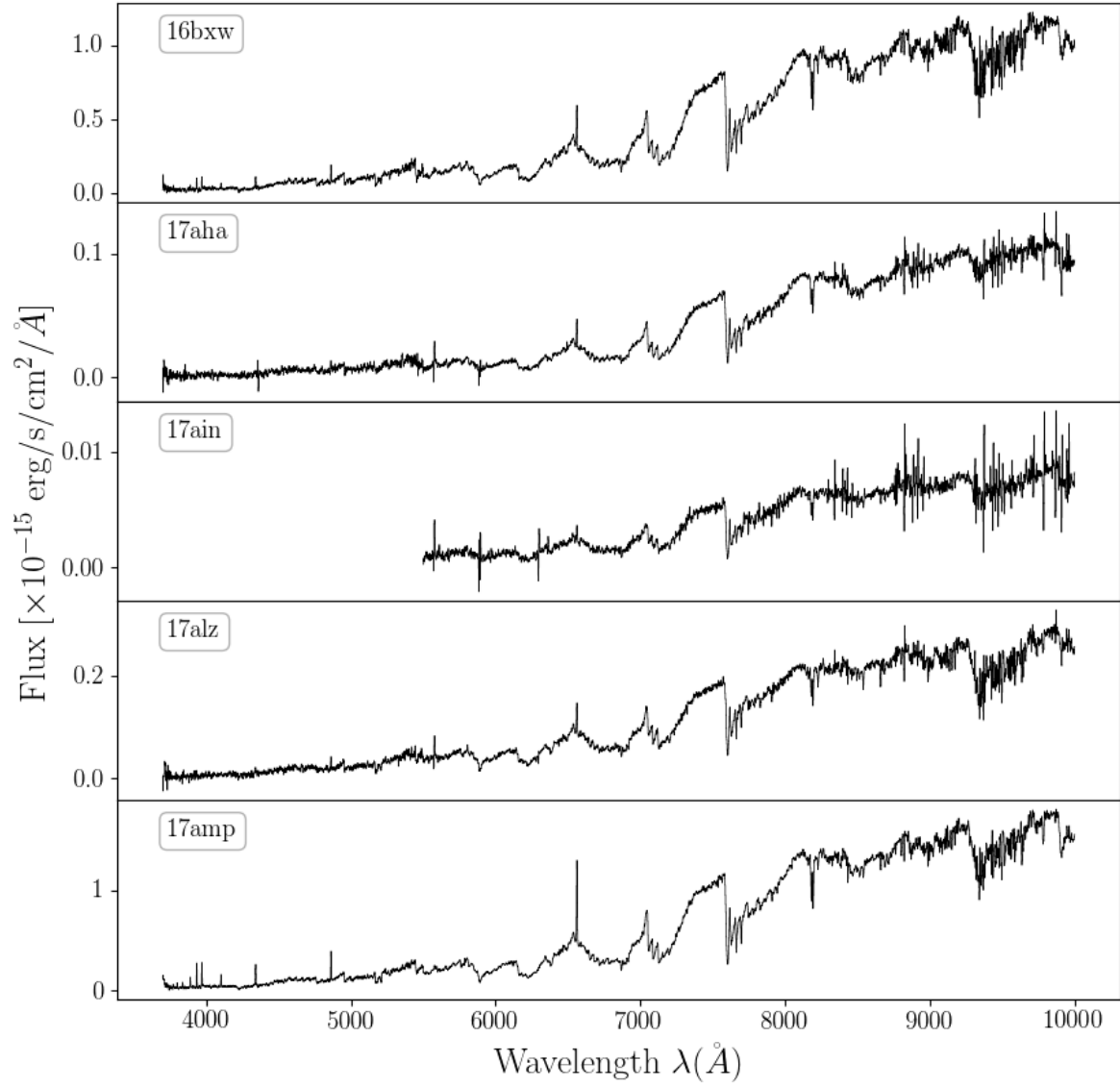
Figure 1. DBSP spectra of five of the M dwarfs in our sample
