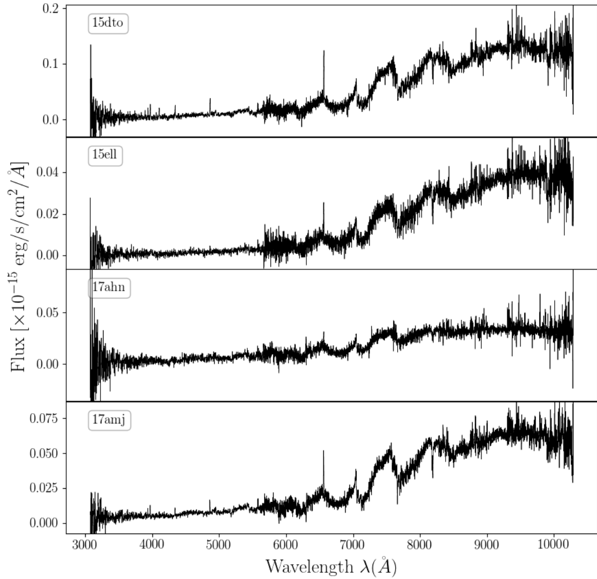
Figure 2. LRIS spectra of four of the M dwarfs in our sample
