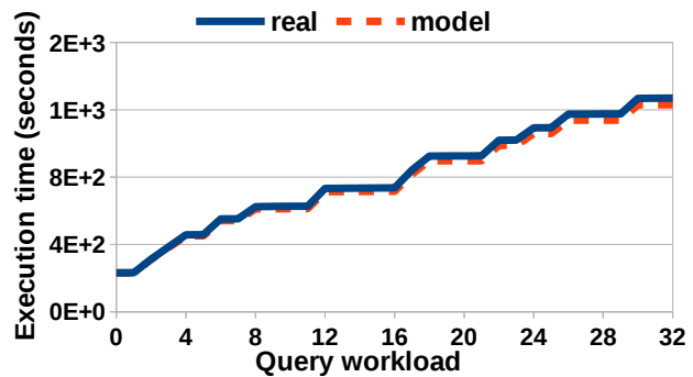
Figure 6: Serial FITS model validation.
