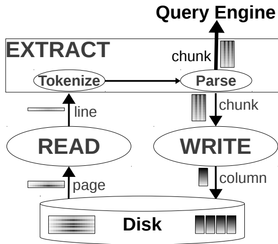
Figure 1: Query processing over raw data.
