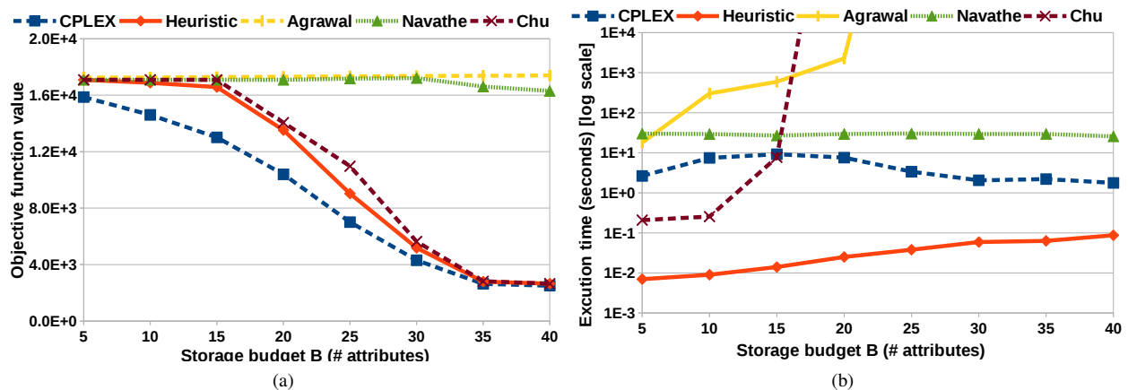
Figure 3: Comparison with CPLEX and vertical partitioning algorithms in objective function value (a) and execution time (b) for serial raw data processing.
