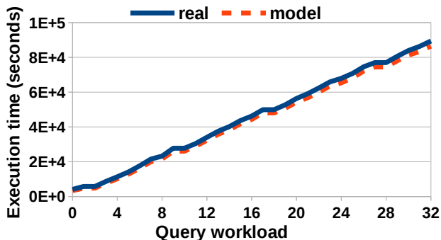
Figure 7: Pipelined JSON model validation.
