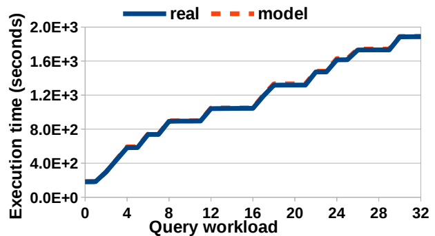
Figure 5: Serial CSV model validation.
