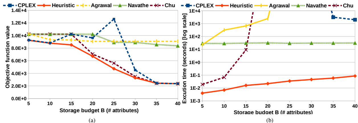
Figure 4: Comparison with CPLEX and vertical partitioning algorithms in objective function value (a) and execution time (b) for pipelined raw data processing.
