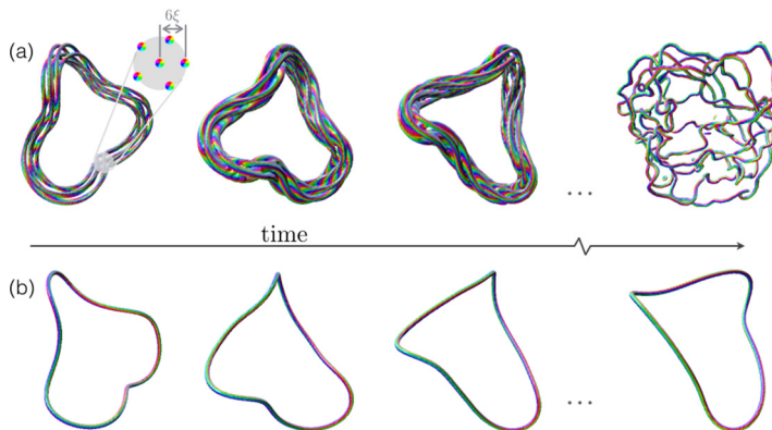
FIG. 3. A threefold helical superfluid vortex bundle [shown in panel (a)] evolving as a coherent structure, rotating as it travels forward, akin to a single threefold helical vortex [shown in panel (b)]. A cross section of the threefold helical superfluid vortex bundle reveals a central vortex and five equally spaced vortices arranged around the central vortex at distance 6\xi (where \xi is the healing length). After a long time, the helical vortex bundle disintegrates (symbolized by the gray dots) and loses its bundle-like structure.
