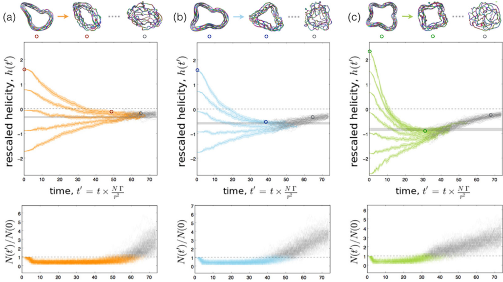
FIG. 5. Helical vortex bundles ( N = 6 ) at different stages of evolution (top row), with the corresponding points in the graphs indicated by colored circles (bundle-like structure preserved), and gray circles (bundles disintegrate). (a) Twofold helical vortex bundles with aspect ratio 0.35, (b) threefold helical vortex bundles with aspect ratio 0.25, and (c) fourfold helical vortex bundles with aspect ratio 0.2. The rescaled helicity h (middle row) for superfluid vortex bundles having the same overall shape (writhe) but different amounts of twist trends toward their initial average writhe (horizontal gray band), before eventually decaying toward zero (gray dotted lines). Bottom panel shows the ratio of the number of vortex filaments at time t' to the initial number of vortex filaments: N(t')/N(0) . For each helical vortex bundle configuration, multiple ( > 10 ) simulations are performed with random Gaussian noise (rms is 2% of the rms radius) added to the initial bundle. The mean rescaled helicity is indicated by the solid lines, and the width of the shaded band around the solid line indicates the standard deviation ( 2\sigma ).
