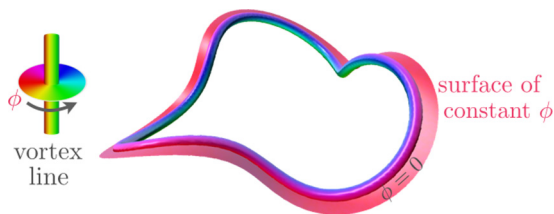
FIG. 1. A threefold helical superfluid vortex and a section of its phase isosurface clipped at a fixed distance from the vortex. The volume occupied by the superfluid naturally separates into such surfaces of constant phase.
