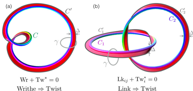
FIG. 2. Vortex lines C and closed curves C' constructed by offsetting vortex lines along a phase isosurface for (a) a writhing (coiling) vortex line C and (b) a pair of linked rings C_1, C_2 . Notice that the presence of either writhe or linking in vortex lines leads to the twisting of the phase isosurface around the vortex lines. The circulation around a closed loop \gamma encircling a vortex line is equal to the change in phase \phi as the loop is traversed, giving a multiple of 2\pi .
