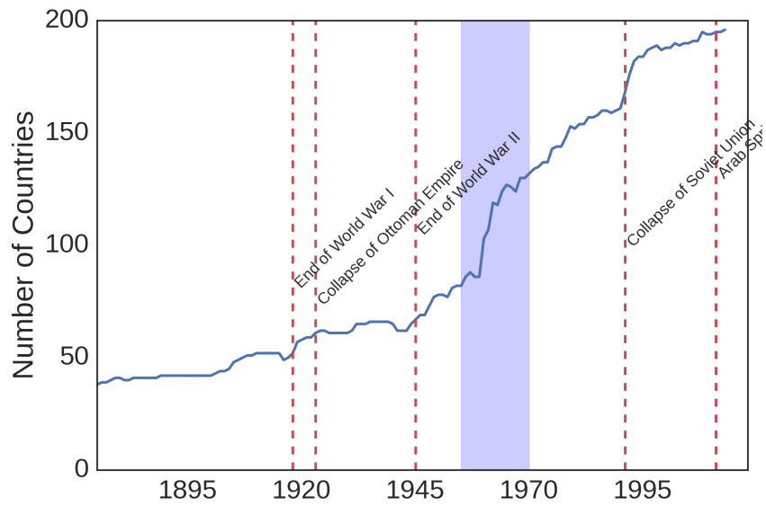
Figure 4: Yearly time series of the number of constitutions in our dataset.
