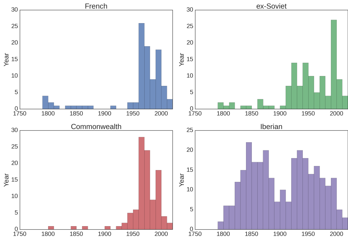
Figure 9: Time Distribution of new Constitution Writing Events
