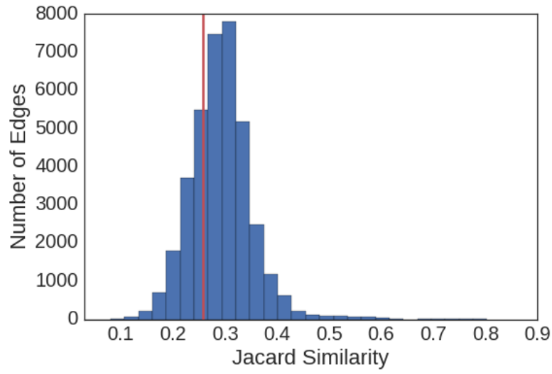
Figure 13: Histogram of Pair-wise Edge Wights in N \times N Jacard Similarity Matrix. Redline indicates the value at which the network becomes disconnected.
