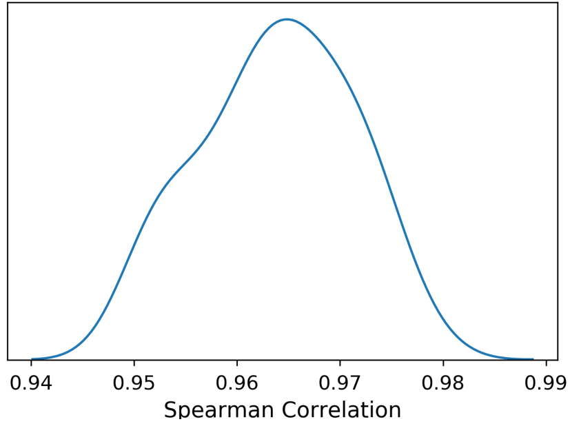
Figure 29: Distribution of n(n-1)/2 = 45 Spearman correlations of rankings over 10 optimisation epochs
