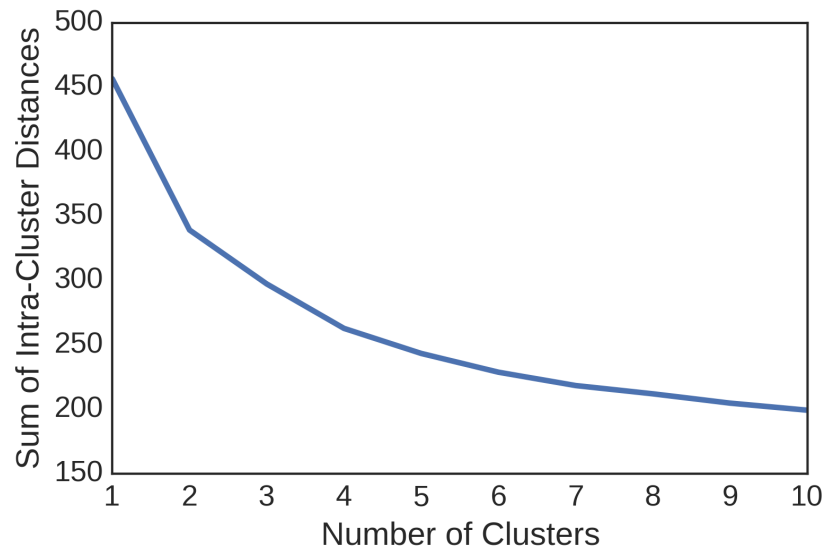
Figure 23: Elbow plot of k-means Clustering of Time-series.
