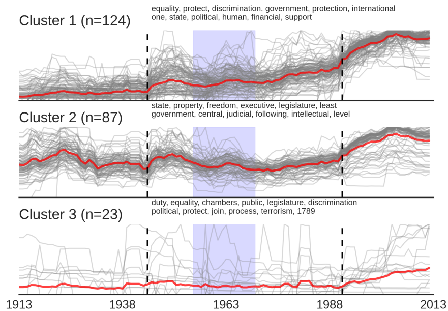
Figure 24: Clusters ( k=3 ) of provisional time series with the mean prevalence of all provisions per year shown in red. Top terms in descriptions of provisions are included.
