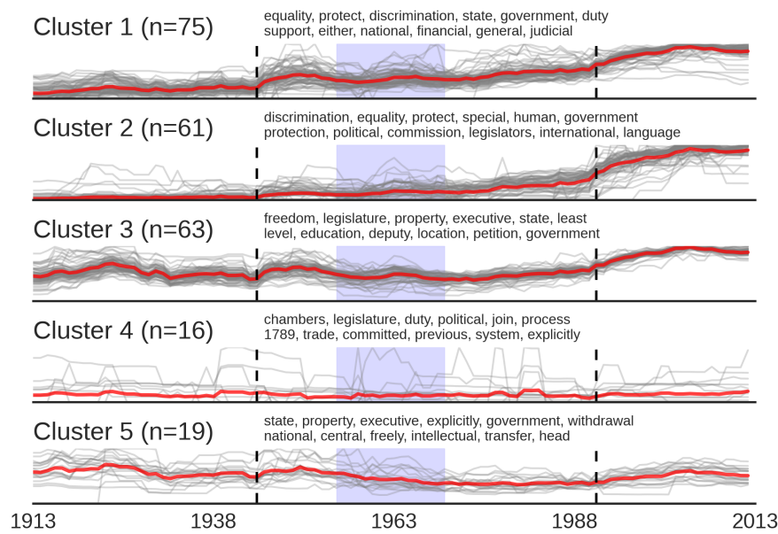
Figure 25: Clusters ( k=5 ) of provisional time series with the mean prevalence of all provisions shown in red. Top terms in descriptions of provisions are included.
