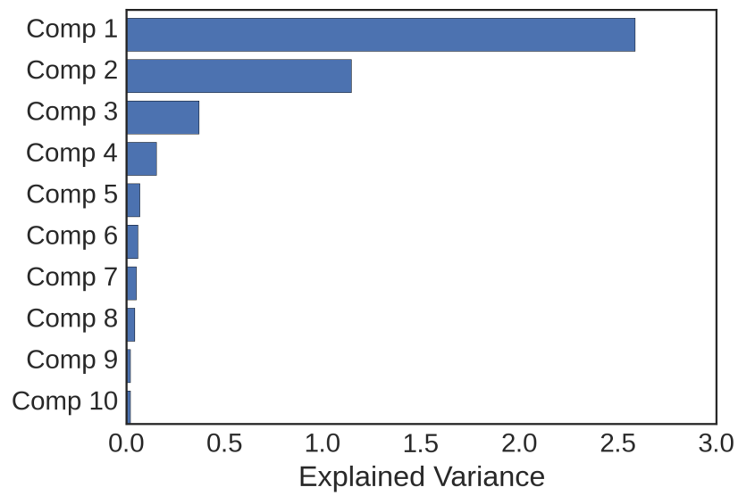
Figure 21: Variance Explained by each Principal Component of Provisional time-series Decomposition.
