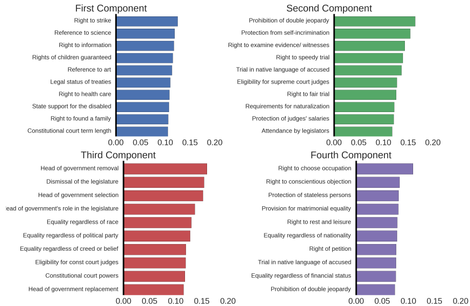
Figure 14: Graphical Representation of Provisions with Largest Projections on first 4 Components under Singular Value Decomposition.
