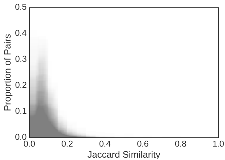
Figure 10: Distribution of Jaccard Similarities for all Provisions
